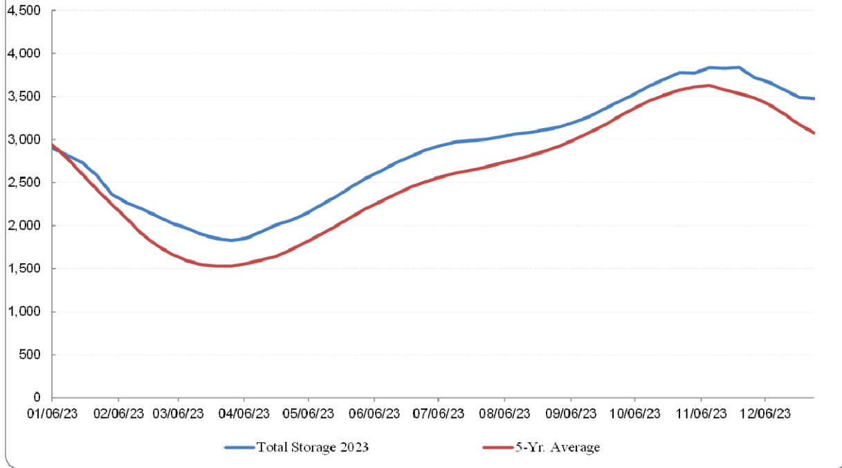
Chart 4-2 Total Working Gas in Storage Comparison of 2023 to Prior 5-Year Average
