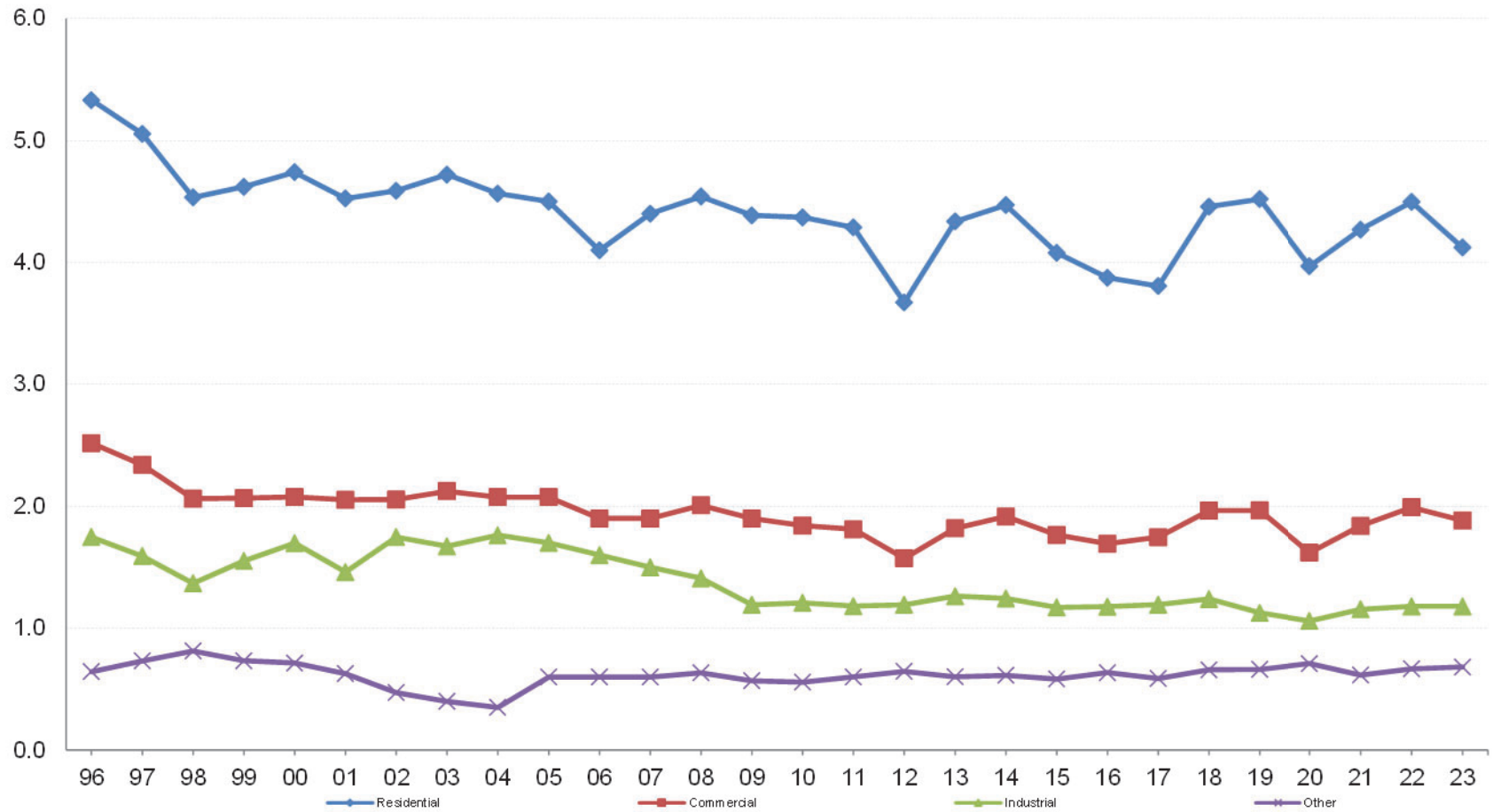
Chart 6-1 ANNUAL NATURAL GAS SALES BY CLASS OF SERVICE (Quadrillion Btu)
